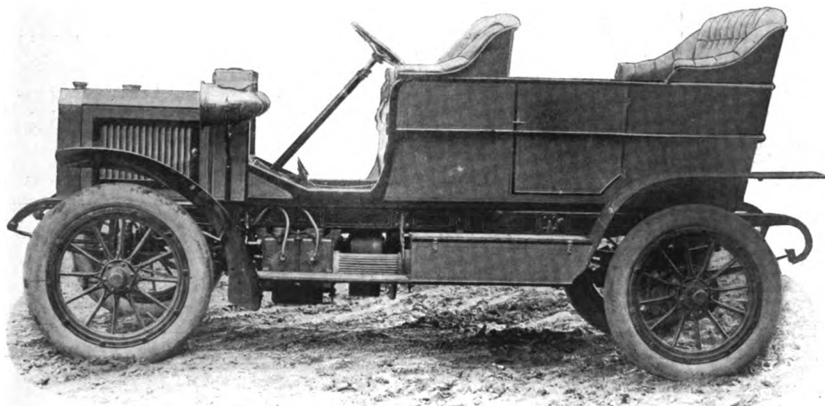
SIDE VIEW OF THE NEW SIDE ENTRANCE STURTEVANT CAR FITTED WITH AUTOMATIC CHANGE SPEED GEAR.
